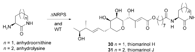
Scheme 4. Mutasynthetic formation of thiomarinols H and J.
